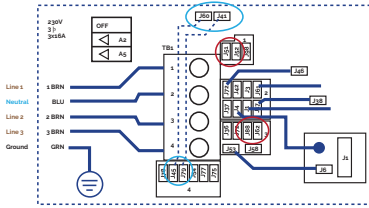
Three-phase line 380V III BP21G1WL
